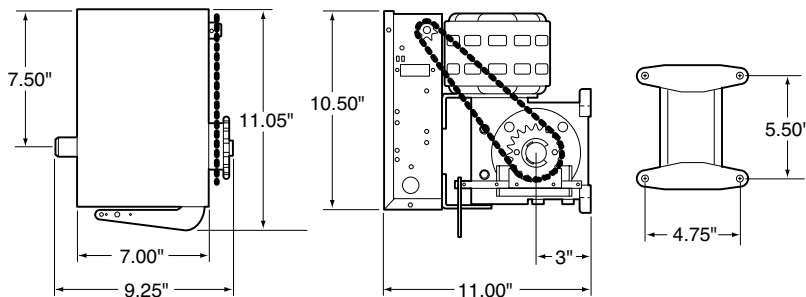
MOUNTING DIMENSIONS
